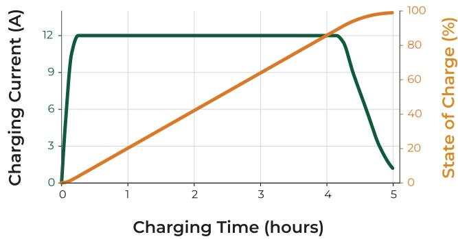
HIO Lithium Charging Curve
