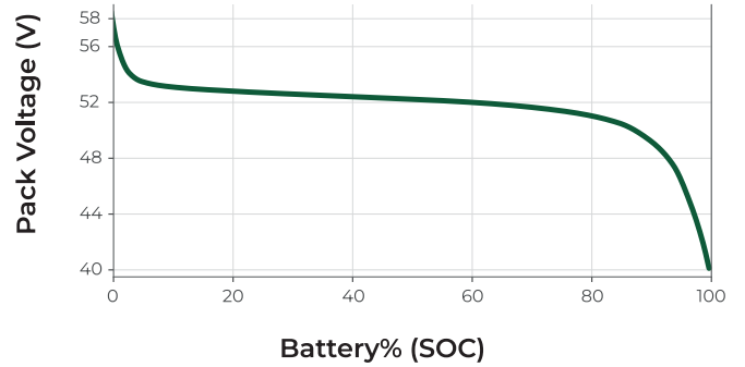
HIO Lithium Voltage Curve
