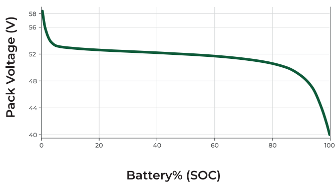
HIO Lithium Voltage Curve
