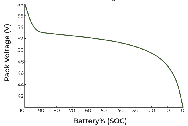
HIO Lithium Voltage Curve
