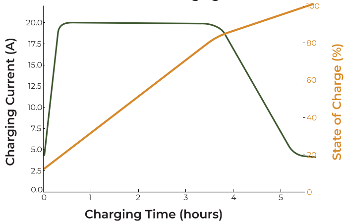
HIO Lithium Charging Curve
