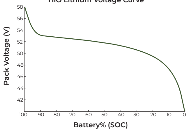
HIO Lithium Voltage Curve
